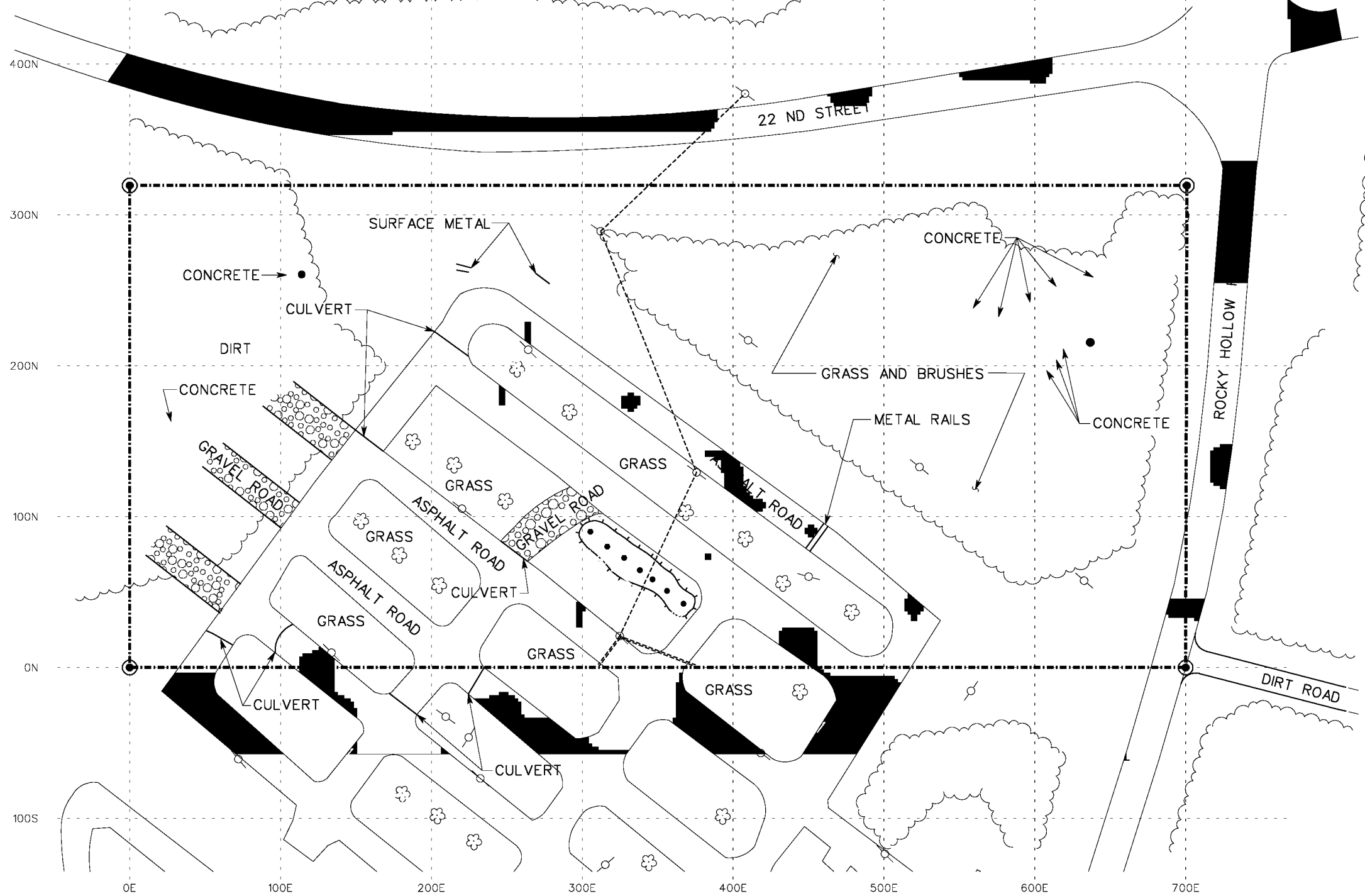
FIGURE 4-1 GROUND SCAR WITH TRENCHES GEOPHYSICAL INTERPRETATION PARCEL 200(7)
